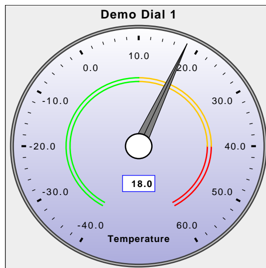
Figure 35.1: Dial Plot
