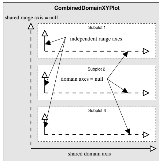
Figure 34.4: CombinedDomainXYPlot axes
