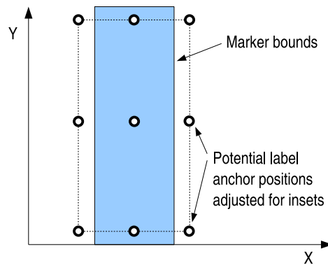
Figure 34.10: Marker insets and the label anchor
