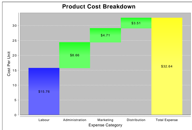
Figure 37.24: A sample chart (see WaterfallChartDemo1.java )
