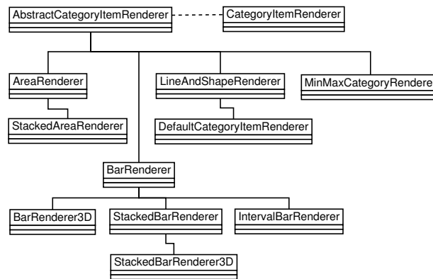
Figure 37.7: Category item renderers
