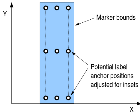
Figure 34.9: Marker insets and the label anchor
