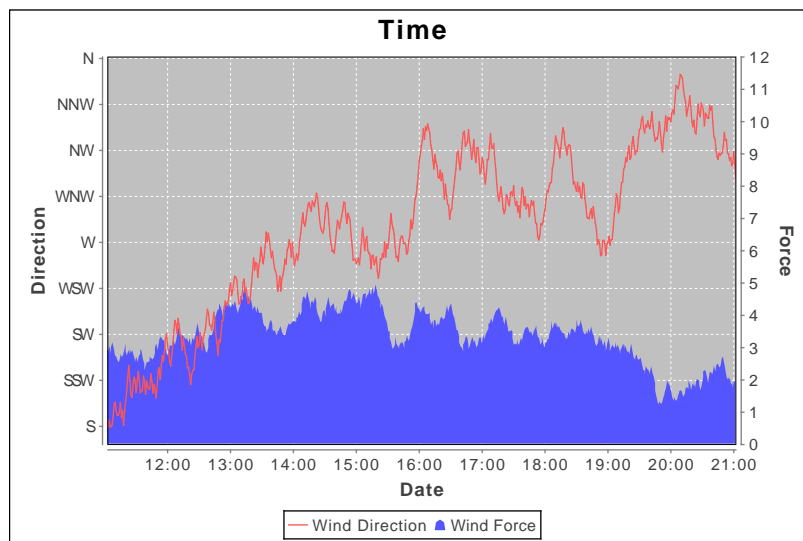
Figure 24.5: A chart that uses the CompassFormat class.
