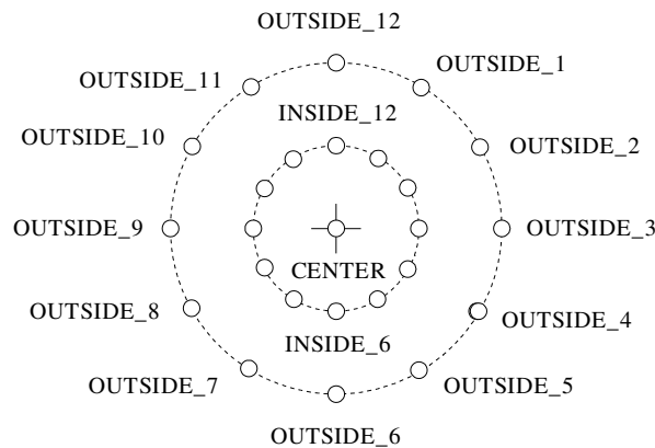
Figure 31.1: The Item Label Anchors
