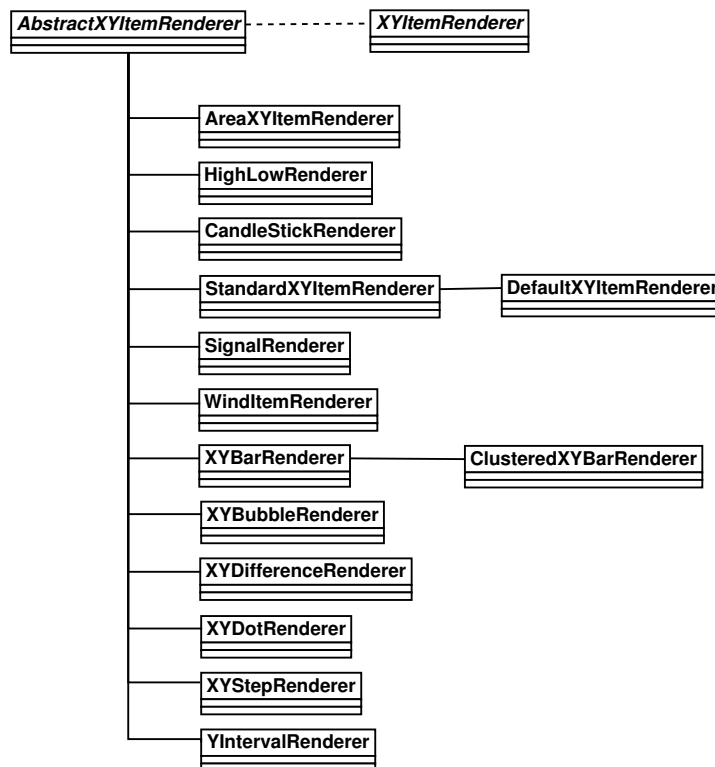
Figure 38.17: Renderer hierarchy
