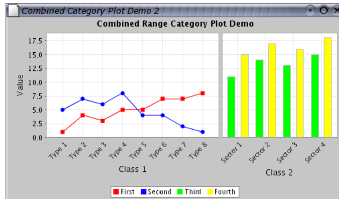
Figure 34.5: A CombinedRangeCategoryPlot
