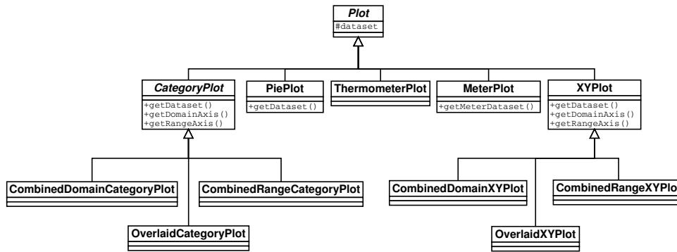
Figure 34.16: Plot classes
