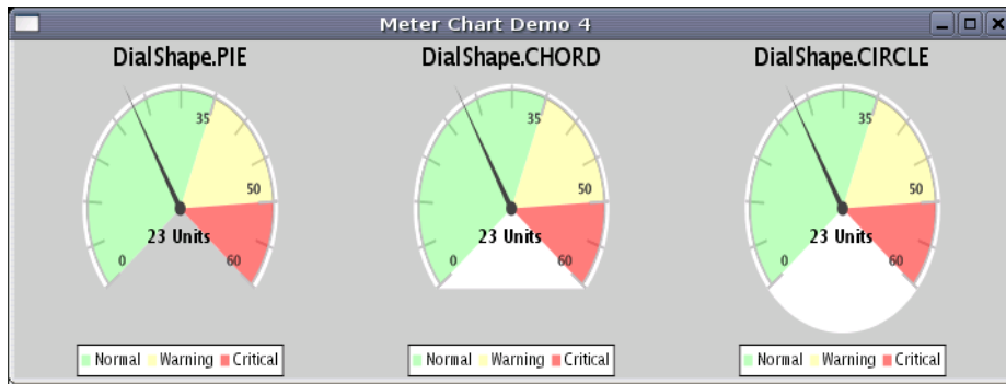
Figure 34.8: DialShape examples
