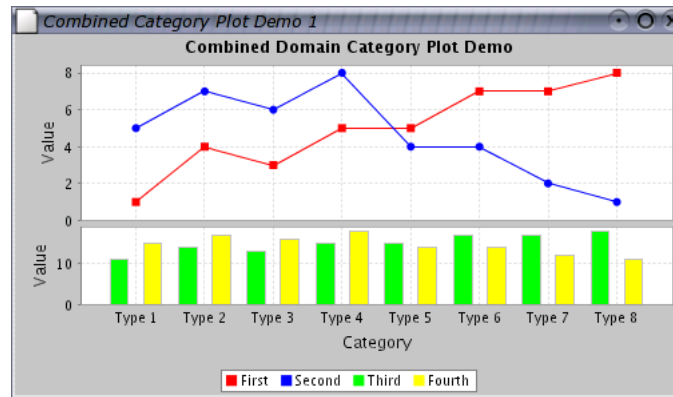
Figure 34.3: A CombinedDomainCategoryPlot
