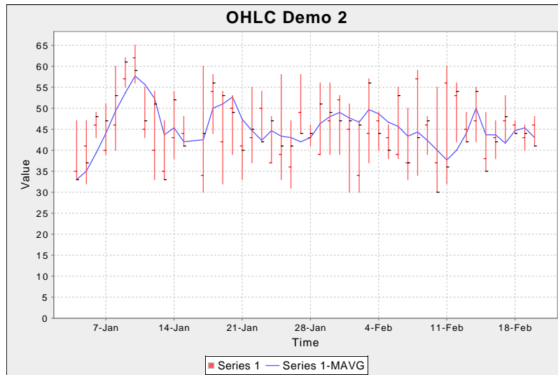
Figure 2.13: A high-low-open-close chart (see HighLowChartDemo2.java )
