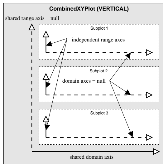
Figure 34.6: CombinedRangeXYPlot axes
